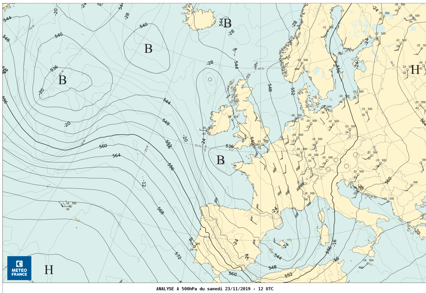
ANALYSE A 500hPa du samedi 23/11/2019 - 12 UTC
