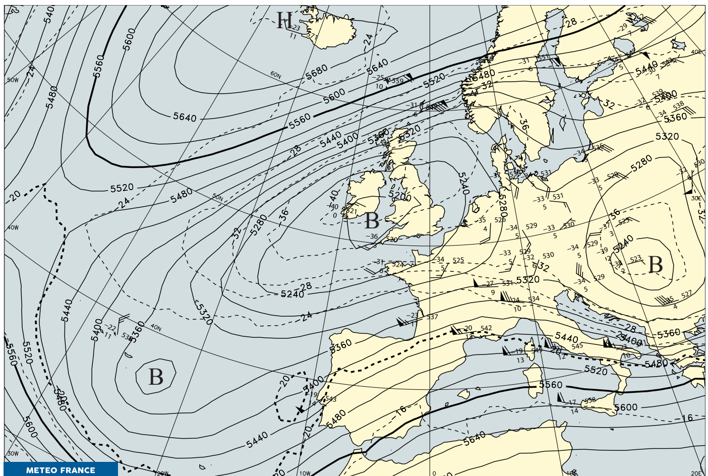
ANALYSE A 500 hPa DU MER 28/02/18 12UTC
